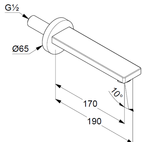
Dimensional drawing
