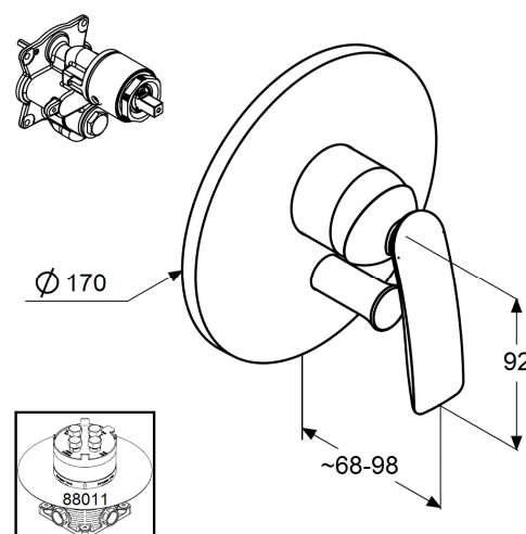
Dimensional drawing
